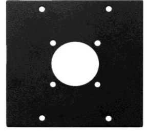
RSP-21SP8 FRONTAL 2 SEGMENTO 1 CONECTOR SPEAKON 8
