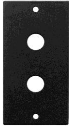
RSP-12RCA FRONTAL 1 SEGMENTO 2 CONECTOR RCA 9.5 MM
