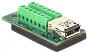
65562 Delock Adapter USB 3.0 / 3.1 PD A female > Terminal Block 14 pin
