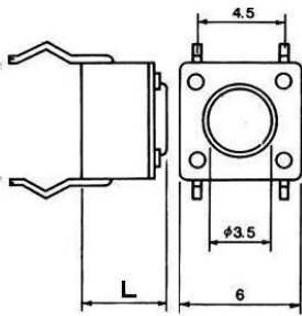
SW0230 PULSADOR TACTO 6x6 mm 12V 50 mA 4 PIN L : 4.30 mm
