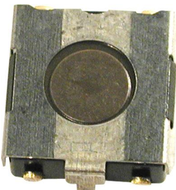
SW0260B PULSADOR TACTO 6x6 mm 12V 50 mA 2 PIN L : 6.00 m
