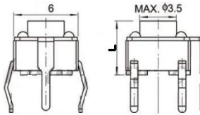
SW0232D PULSADOR TACTO 6x6 mm 12V 50 mA 5 PIN L : 7.30 mm
