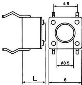
SW0230E PULSADOR TACTO 6x6 mm 12V 50 mA 4 PIN L : 8.00 mm
