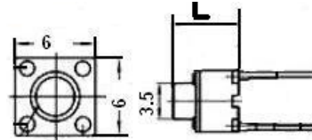
SW0260 PULSADOR TACTO 6x6 mm 12V 50 mA 2 PIN L : 4.30 m
