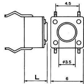
SW0230D PULSADOR TACTO 6x6 mm 12V 50 mA 4 PIN L : 7.30 mm
