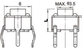
SW0232A PULSADOR TACTO 6x6 mm 12V 50 mA 5 PIN L : 5.00 mm
