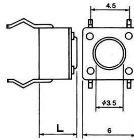
SW0230B PULSADOR TACTO 6x6 mm 12V 50 mA 4 PIN L : 7.00 mm
