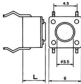
SW0230A PULSADOR TACTO 6x6 mm 12V 50 mA 4 PIN L : 5.00 mm
