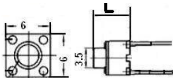
SW0260B PULSADOR TACTO 6x6 mm 12V 50 mA 2 PIN L : 6.00 m
