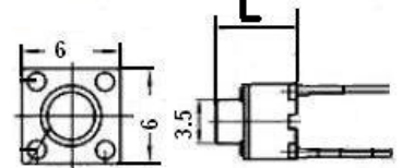
SW0260A PULSADOR TACTO 6x6 mm 12V 50 mA 2 PIN L : 5.00 m
