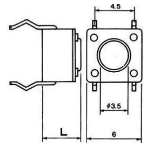
SW0230H PULSADOR TACTO 6x6 mm 12V 50 mA 4 PIN L : 19.00 mm
