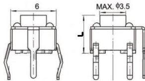
SW0232C PULSADOR TACTO 6x6 mm 12V 50 mA 5 PIN L : 9.30 mm
