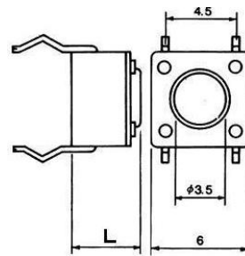
SW0230G PULSADOR TACTO 6x6 mm 12V 50 mA 4 PIN L : 17.00 mm
