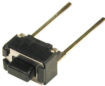
SW0244P PULSADOR TACTO 3x6 mm 12V 50 mA L : 5.00 mm
