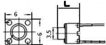
SW0260C PULSADOR TACTO 6x6 mm 12V 50 mA 2 PIN L : 9.00 m
