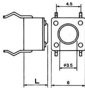
SW0230F PULSADOR TACTO 6x6 mm 12V 50 mA 4 PIN L : 12.50 mm
