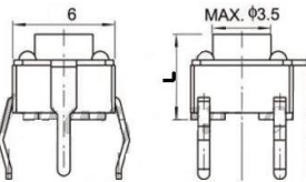
SW0232 PULSADOR TACTO 6x6 mm 12V 50 mA 5 PIN L : 4.30 mm
