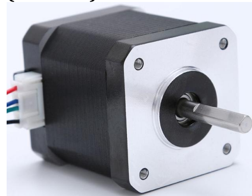
DMT006 MOTOR PASO A PASO 42BYGH48-23D 48 mm 1.7A/0.55 N.M (NEMA17)
