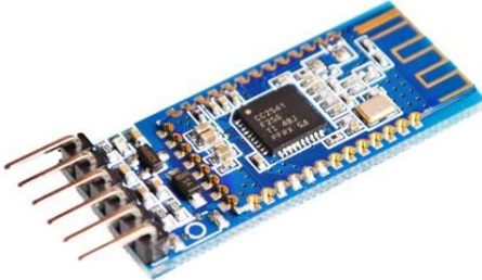
MD9029 MODULO BLUETOOTH 4.0
