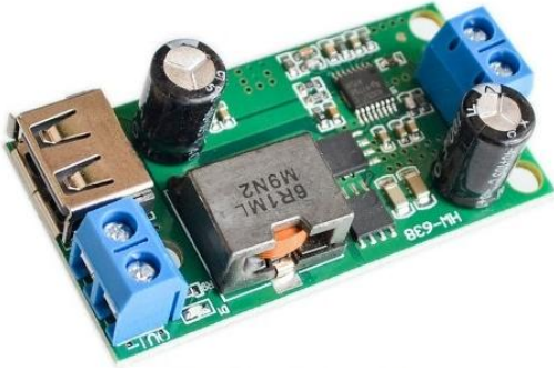
MD9060 MODULO DC-DC STEP DOWN 3-35 VDC 6A LTC1831
