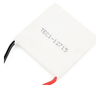
PT12715 CELULA PELTIER 12V 15A 180W 40x40 mm
