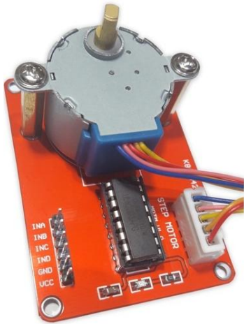
CP0095 MOTOS PASO A PASO + DRIVER ULN2003
